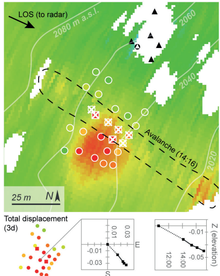
Figure 5: Field setup of the validation with total station and GPS boxes. The total station is located at (782494/188159). The results of the total station measurements were calculated for the observation period after the avalanche and were converted to LOS velocity. The results are plotted as color coded points on top of the GPRI LOS velocity map of the same observation period (14:16-17:00 UTC) with the same color coding. Below the map, the uncorrected total station displacement values and an example of the displacement vector are given.
