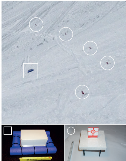
Figure 5: Field setup of the validation with total station and GPS boxes. The total station is located at (782494/188159). The results of the total station measurements were calculated for the observation period after the avalanche and were converted to LOS velocity. The results are plotted as color coded points on top of the GPRI LOS velocity map of the same observation period (14:16-17:00 UTC) with the same color coding. Below the map, the uncorrected total station displacement values and an example of the displacement vector are given.
