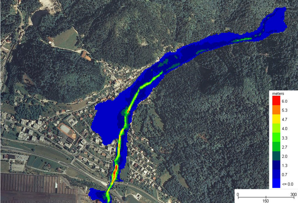
Fig. 4 Maximum flow depths using classical DEM5
