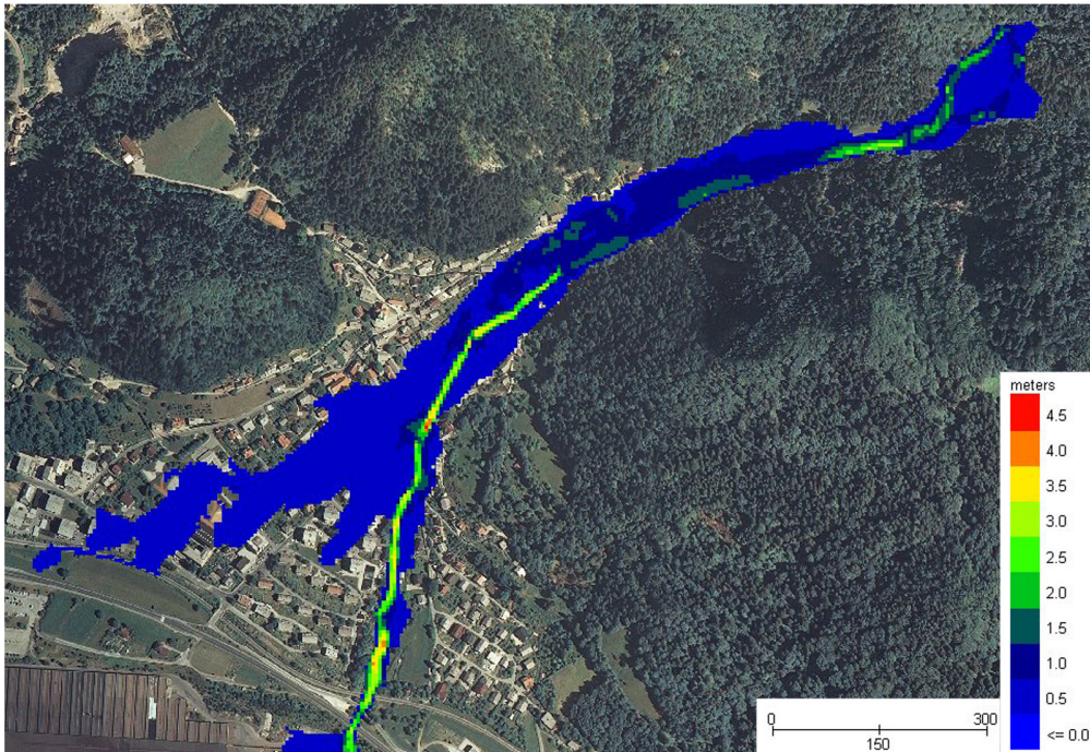
Fig. 1 Maximum depths using higher Manning coefficient for representing structures.
