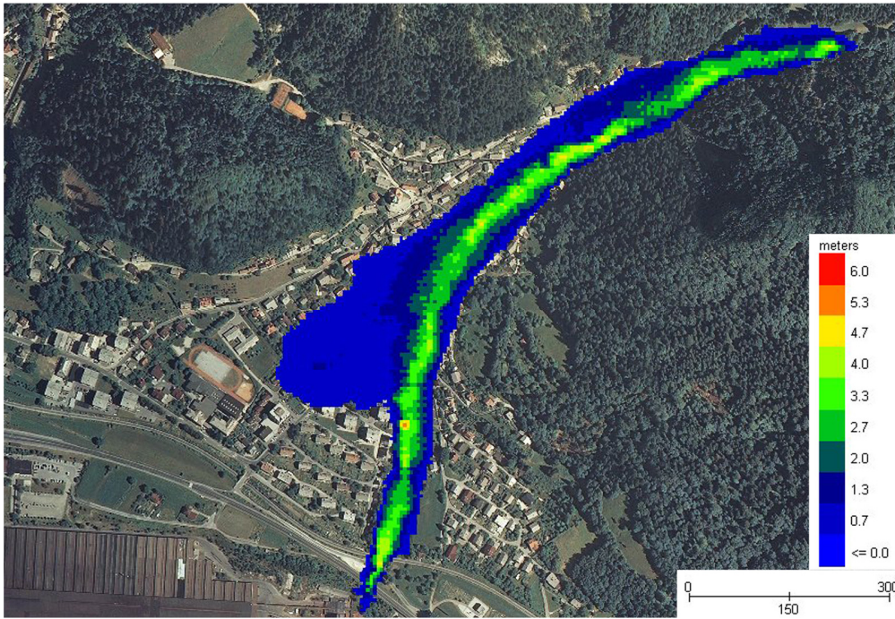
Fig. 5 Maximum flow depths using classical DEM12.5
