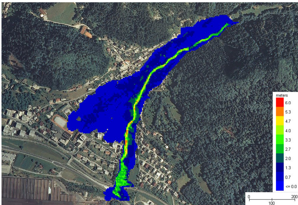
Fig. 6 Maximum flow depths using DEM0.5 (original LiDAR data)
