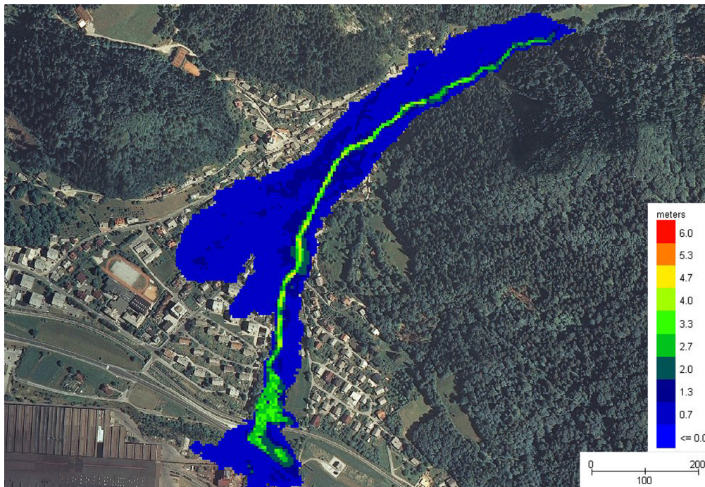
Fig. 7 Maximum flow depths using DEM5 (re-sampled LiDAR data)
