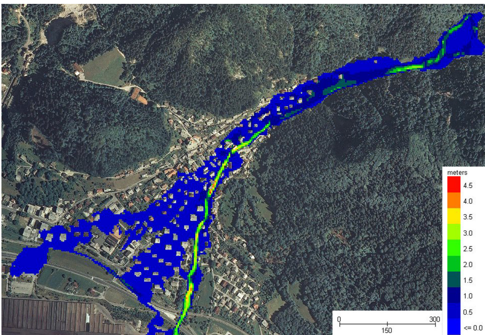
Fig. 2 Maximum depths using blocked ("dry") cells for representing structures.
